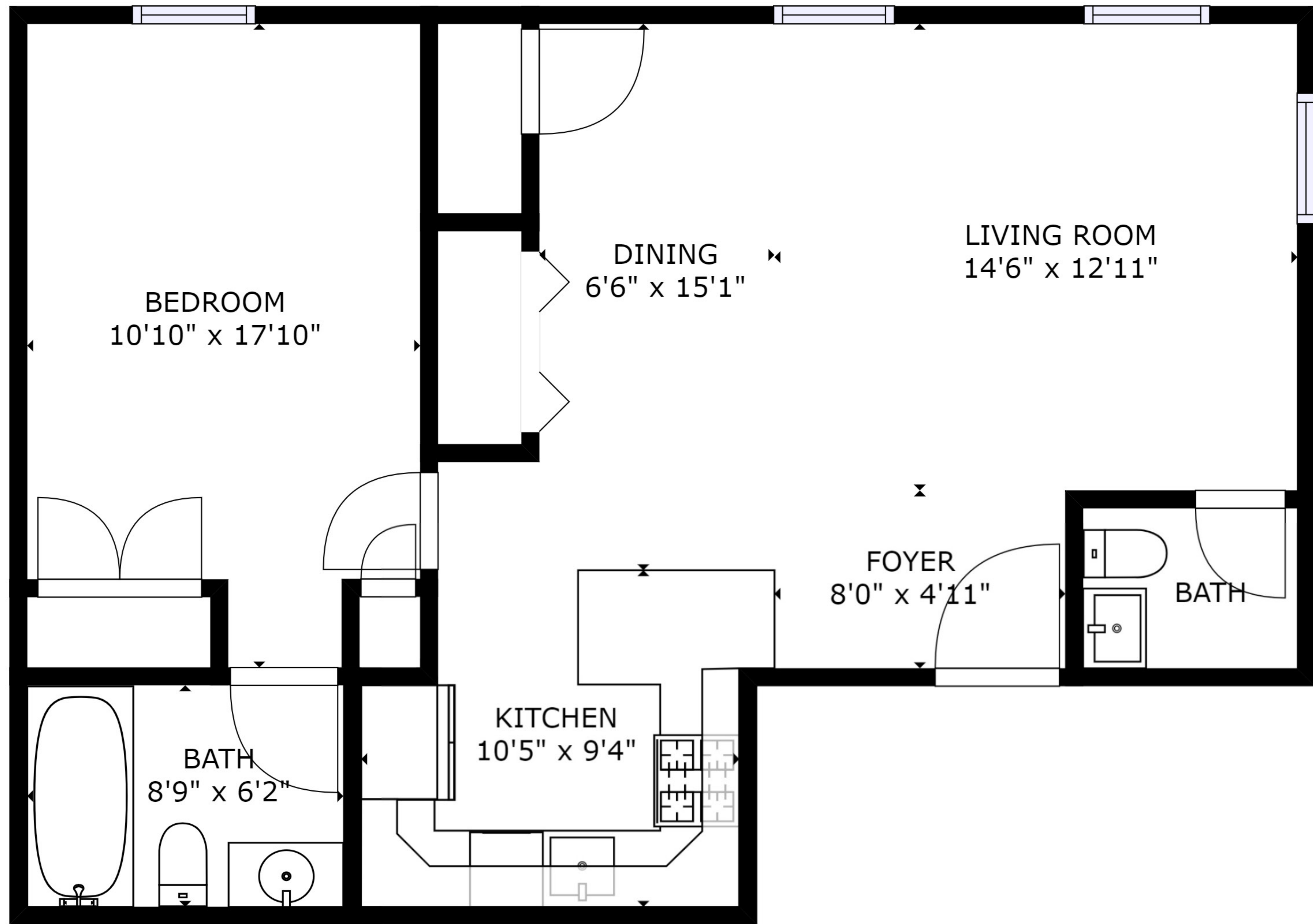
FLOOR 1
